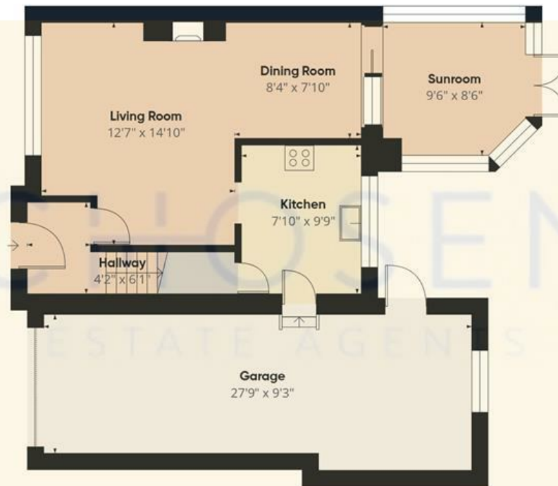
Floor 0
